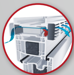
GECCO 4 geopend
